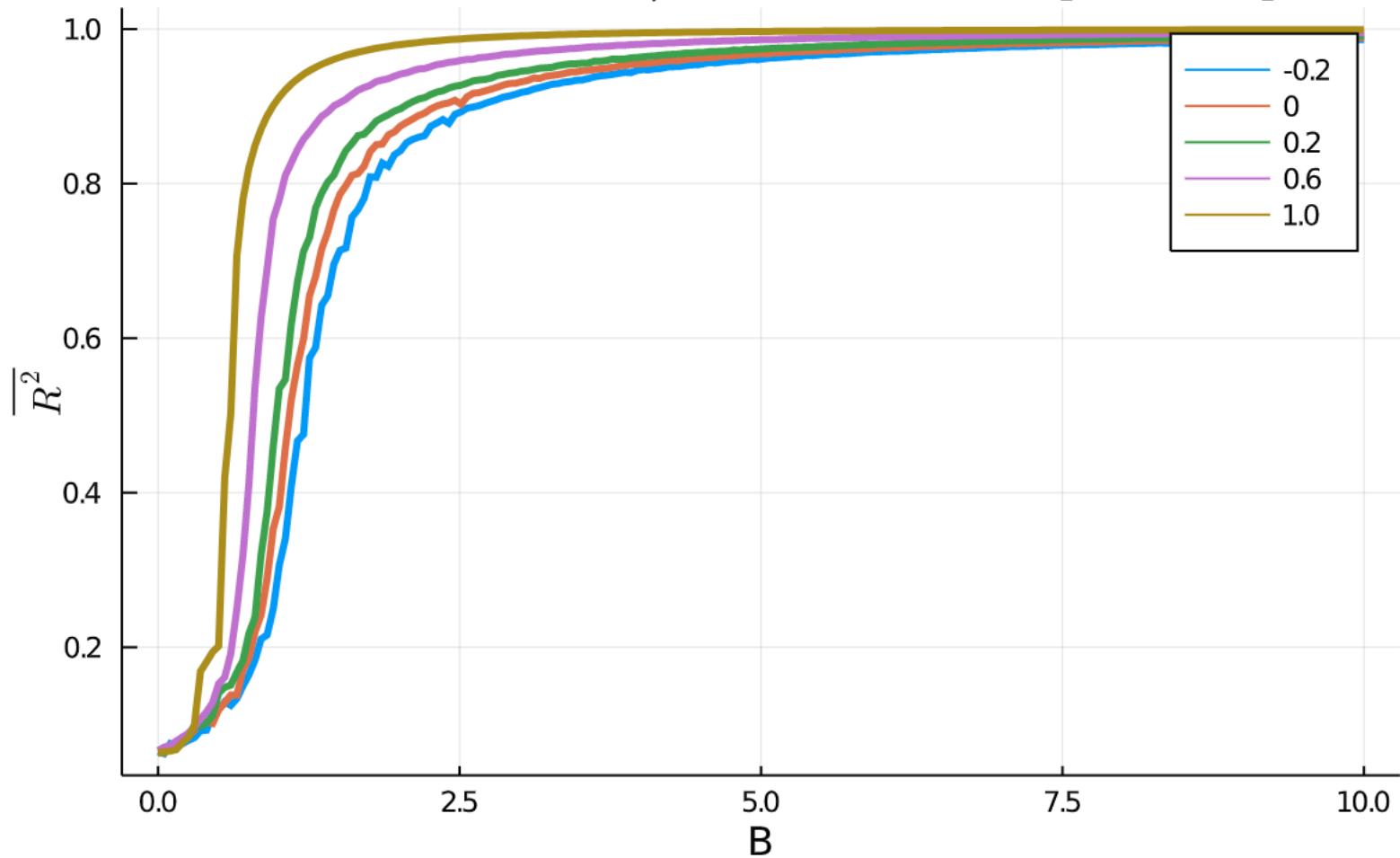
\overline{R^2} vs. B for Several \rho for 16-Node Complete Graph
